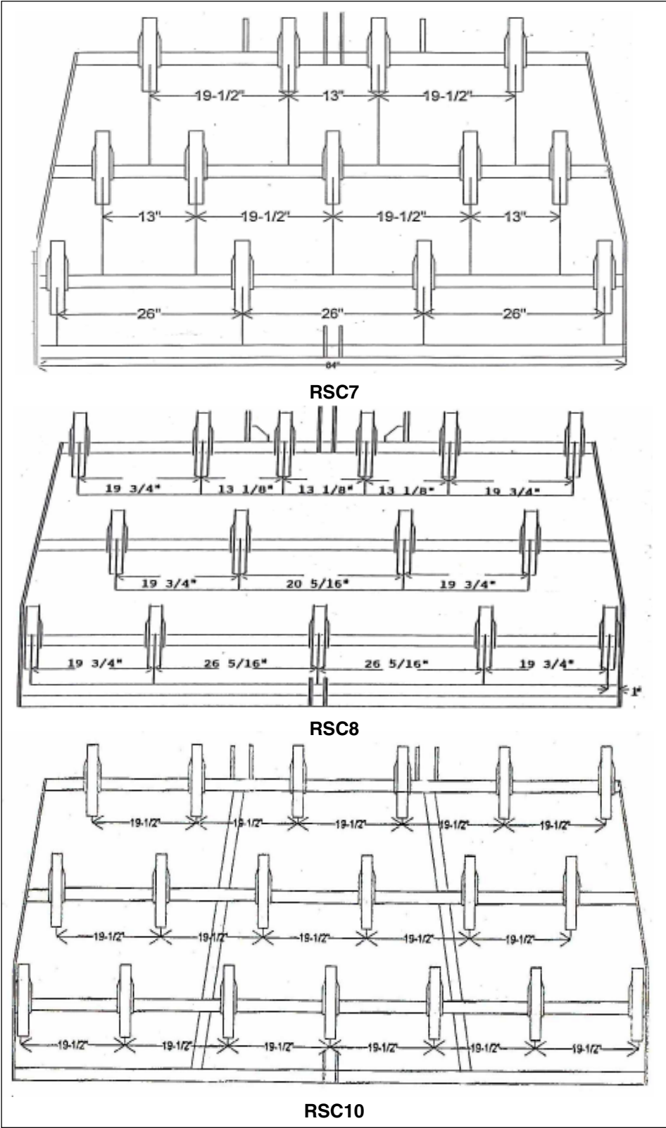
Fig. 14 TINE LOCATIONS
