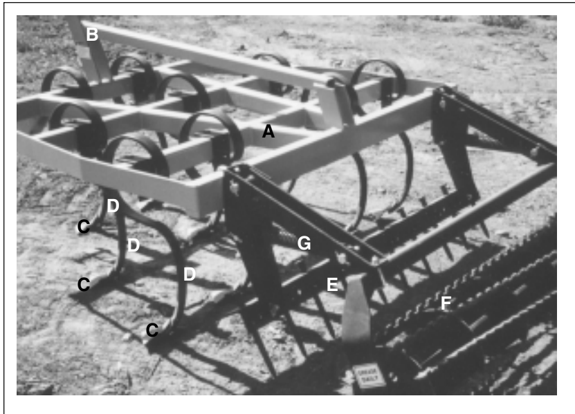
Fig. 1 MACHINE COMPONENTS
