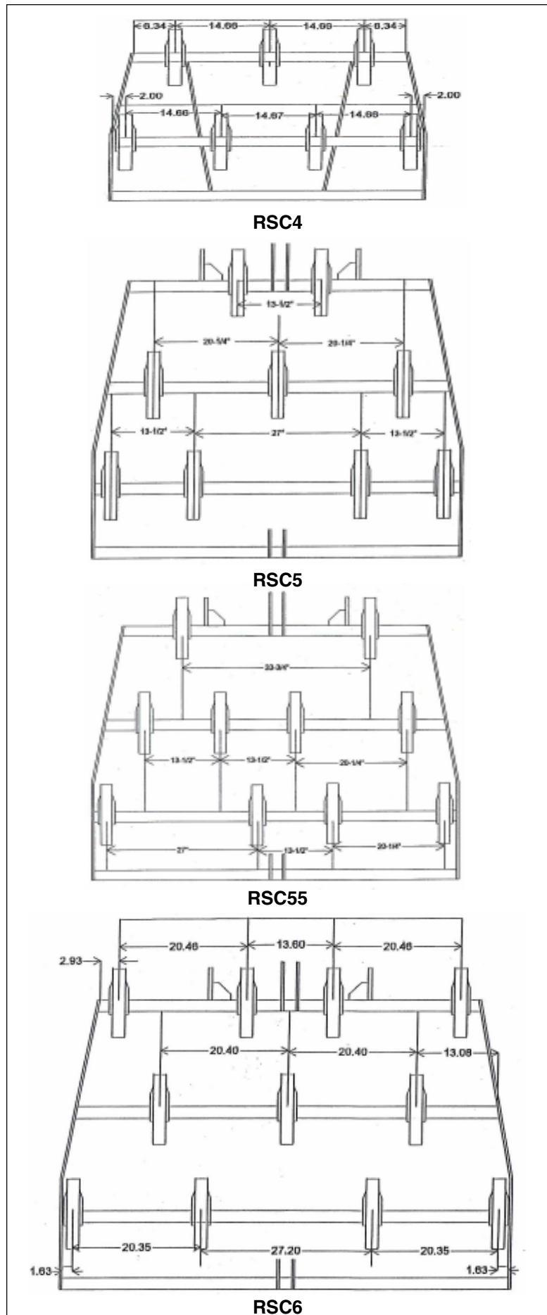
Fig. 13 TINE LOCATIONS
