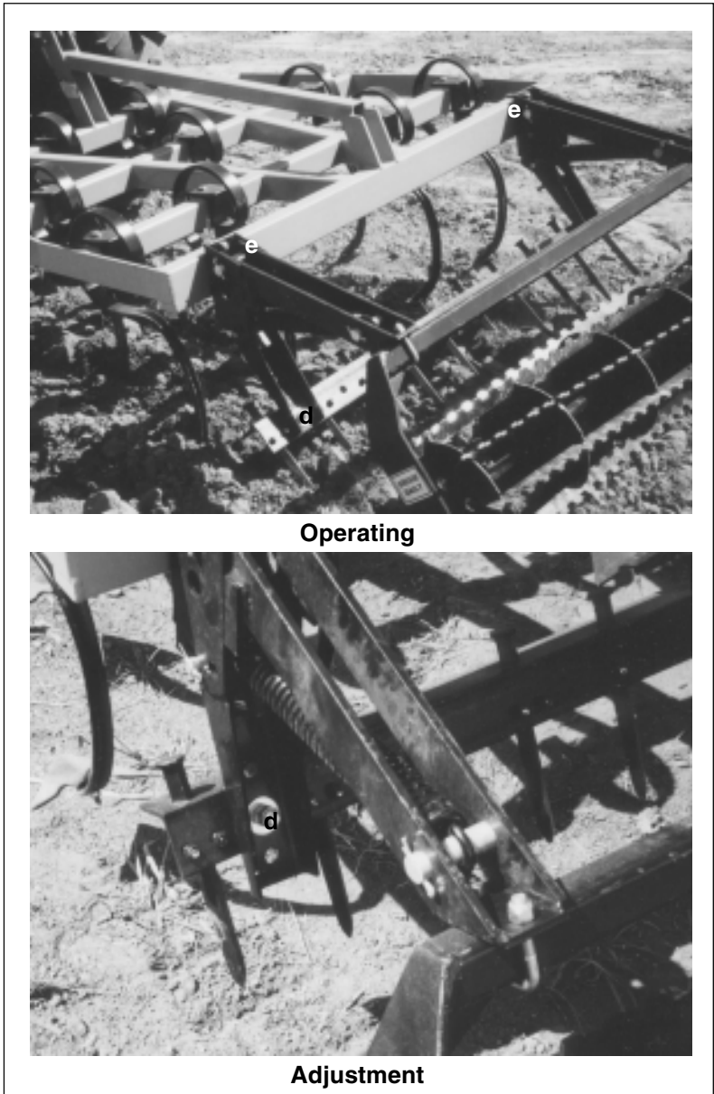
Fig. 4 HARROW BAR/ROLLER
