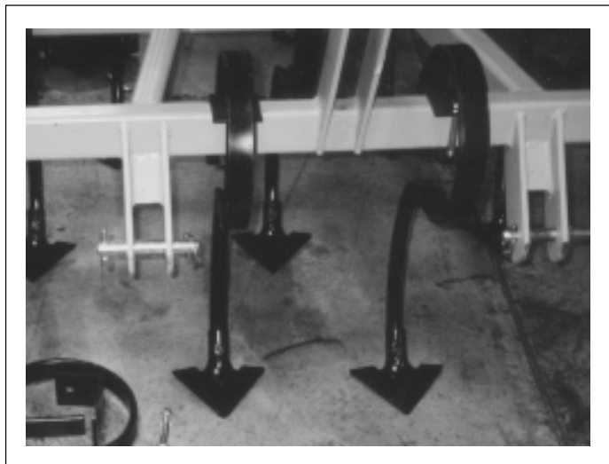
Fig. 12 TIGHTENING
