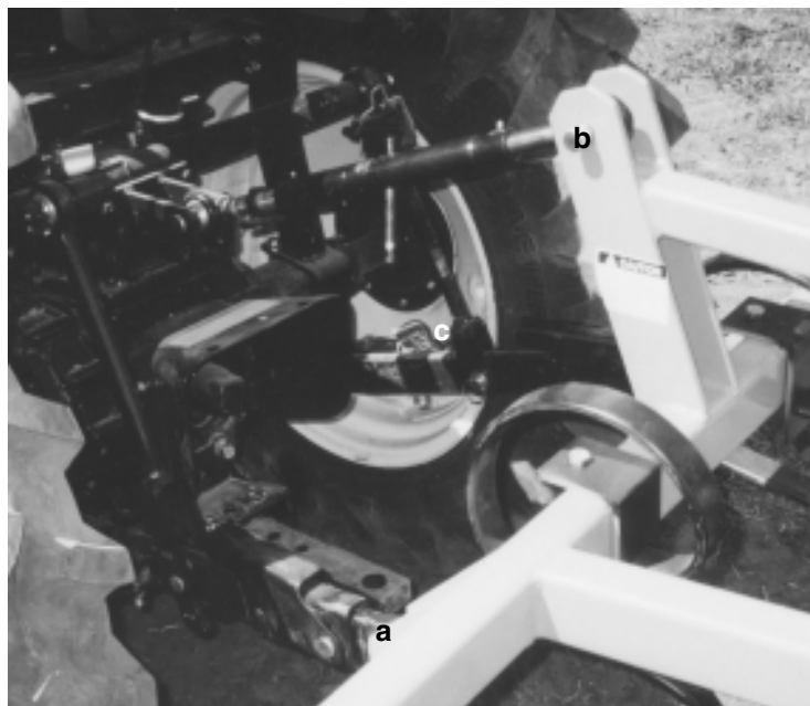
Fig. 2 ATTACHED
