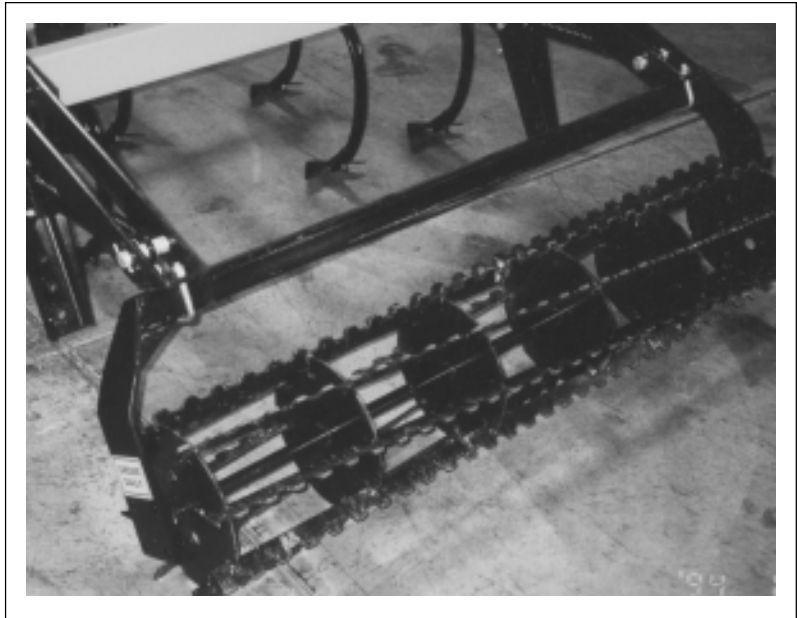
Fig. 17 CRUMBLER ROLLER
