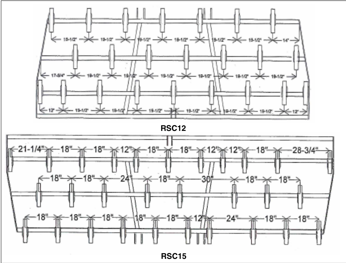
Fig. 15 TINE LOCATIONS
